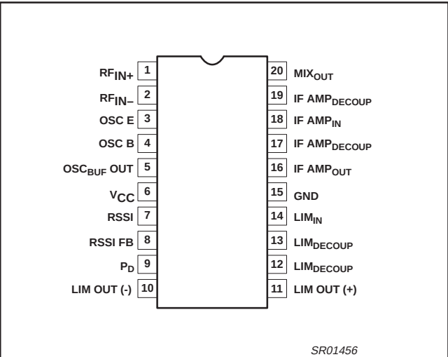
Figure 1. Pin Configuration
